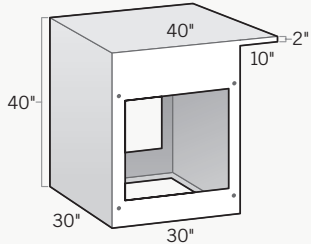
Bar-Height Cabinet with 10" Cantilever Backside 30"D x 30"L x 36"H
