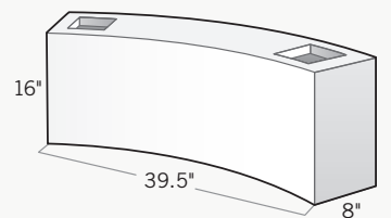
Curved Seating Wall (1/8 Circle) 8"D x 39.5"L x 16"H Curved seating wall has a 51" radius from the center point to the inside edge, perfect for pairing with our round fire pit.
