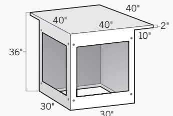
90° Corner Cabinet with 10" Cantilever on Two Sides 30"D x 30"L x 36"H
