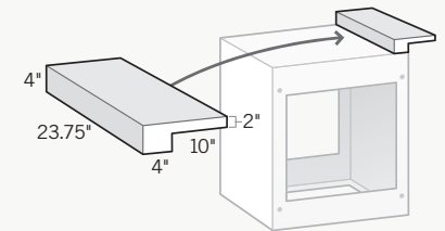
Straight Raised Backsplash Creates 4" high raised backsplash (23.75" long) with 10" cantilever and 14" counter surface. Requires 3 bolts for mounting (not included).
