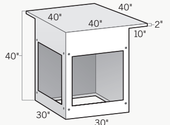
Bar-Height 90° Corner Cabinet with 10" Cantilever on Two Sides 30"D x 30"L x 40"H
