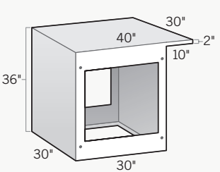
Cabinet with 10" Cantilever Backside 30"D x 30"L x 36"H
