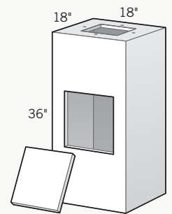
Column with End Cap 18"D x 18"L x 36"H Instantly build perfect stone or brick columns. Ships with access panel. Designed with top and bottom flange for attaching masonry anchor or bolting.
