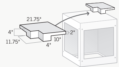
Corner Raised Backsplash Creates a 4" high raised corner backsplash with a 10" cantilever; connects to straight raised backsplash for L-shaped configurations. Requires 2 bolts for mounting (not included).
